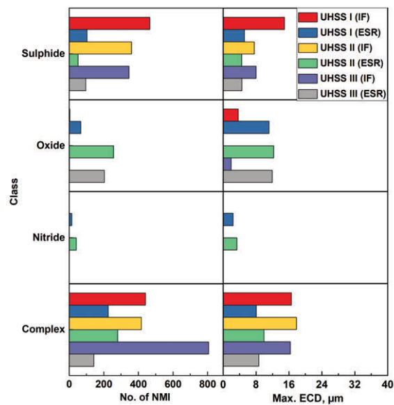
Figure 7. Number of NMIs and maximum ECD of each class of NMI without and with ESR
