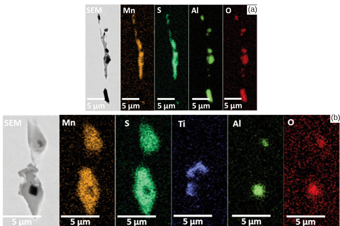
Figure 10. EDS maps of deformed inclusions in UHSS I: (a) \text{MnS}.\text{Al}_2\text{O}_3 (b) \text{MnS}.\text{TiN}.\text{Al}_2\text{O}_3
