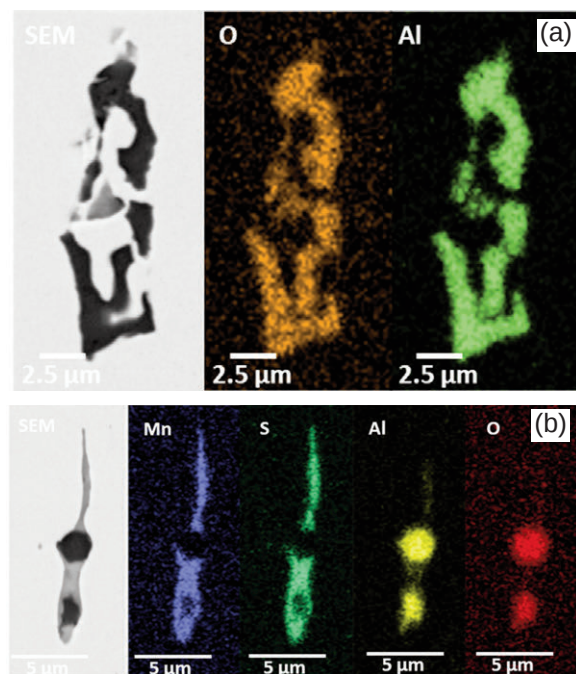
Figure 13. EDS maps of deformed inclusions: (a) \text{Al}_2\text{O}_3 (b) \text{MnS}.\text{Al}_2\text{O}_3
