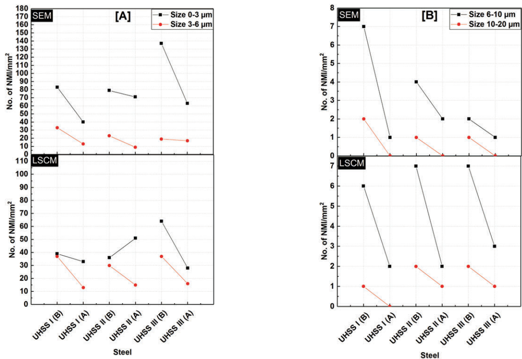
Figure 3. Number of NMIs per mm² in UHSS I, II and III without and with ESR. Results from SEM and LSCM investigations; [A]: size ranges 0-3 μm and 3-6 μm; [B]: size ranges 6-10 μm and 10-20 μm
