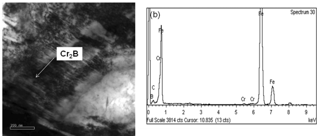
Figure 11. TEM micrographs for steel 1 (a) Cr_2B at a cooling rate 30\text{ }^{\circ}C/s (b) EDS spectrum of taken on these precipitates showing Cr and B peaks
