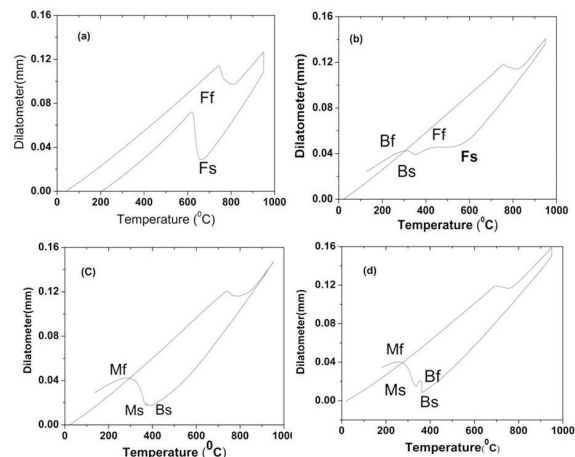
Figure 4. Dilatometric curves representing the phase transformation at cooling rate (a) 1 °C/s (b) 10 °C/s, (c) 20 °C/s, (d) 30 °C/s for steel 1. (Fs-ferrite start, Ff-Ferrite finish, Bs-Bainite start, Bf-Bainite finish, Ms-Martensite start, Mf-Martensite finish temperatures)
