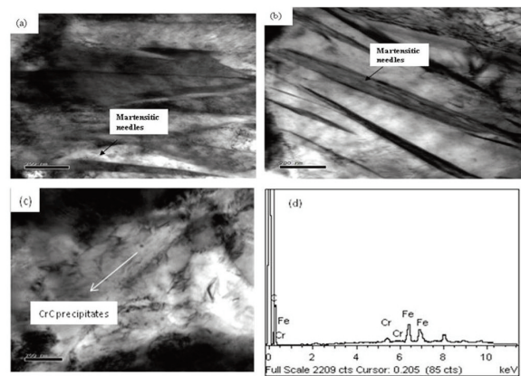
Figure 9. TEM micrographs for steel 2 at various cooling rates showing (a) presence of martensitic needles at a cooling rate 20 °C/s (b) presence of martensitic needles at cooling rate of 30 °C/s (c) presence of globular carbides (d) EDS spectrum of taken on these precipitates showing Cr and C peaks
