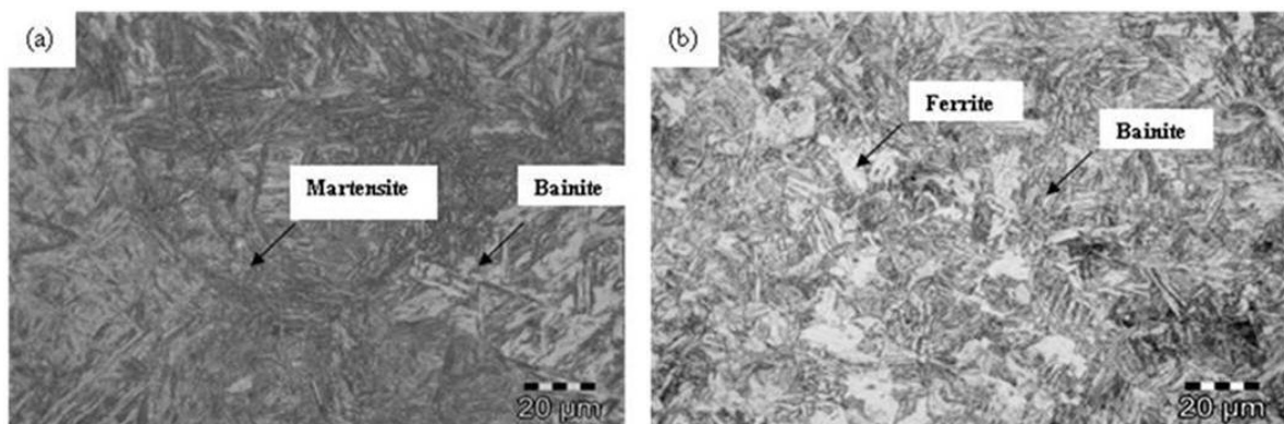
Figure 12. Optical microstructures of steel 1(a) Undeformed, cooled at a rate of 30\text{ }^{\circ}C/s to ambient temperature (b) Deformed upto 50% and cooled at a rate of 30\text{ }^{\circ}C/s to ambient temperature
