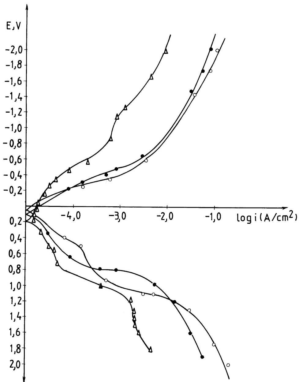
Figure 2. Potentiodynamic curves for steel Č 4583 in tested corrosive media where: (o) E_r = 45 \text{ mV} , ( \bullet ) E_r = 100 \text{ mV} , ( \Delta ) E_r = 200 \text{ mV} , i.e. (o) - 50 wt. % suspension, ( \bullet ) 10 wt. % solution i ( \Delta ) 1 wt. % solution.
