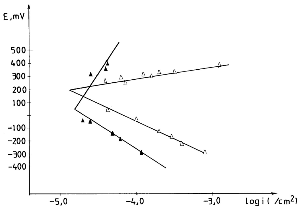
Figure 6. Graphical determination of the corrosion current in the 50wt.% \text{Ca}(\text{OCl})_2 suspension where: ( \Delta ) - steel Č 4574, ( \blacktriangle ) steel Č 4583.
