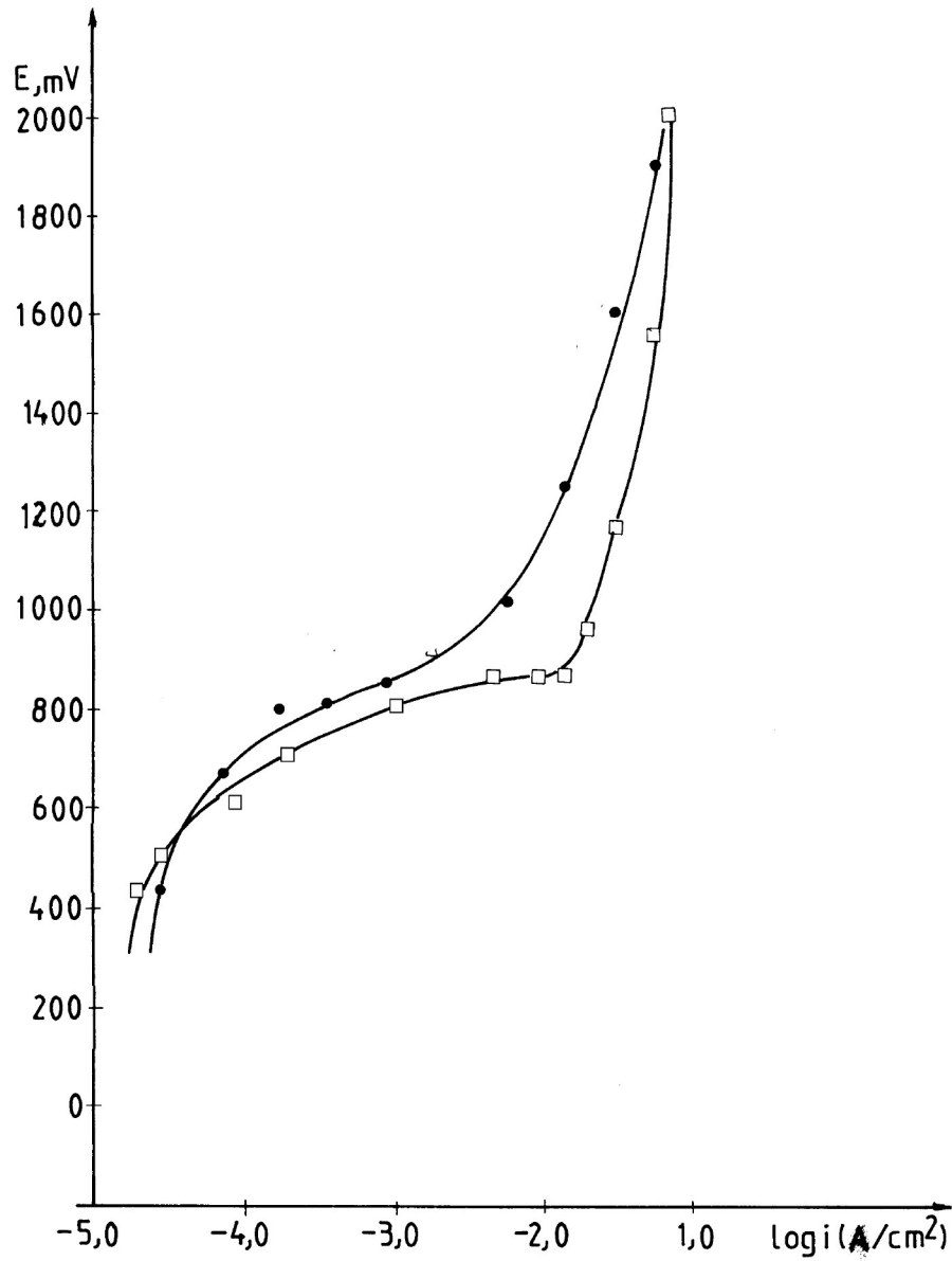
Figure 4. Anode polarization curves in the 10 wt.% \text{Ca(OCl)}_2 suspension where: (●) - steel Č 4574, (□) steel Č 4583.
