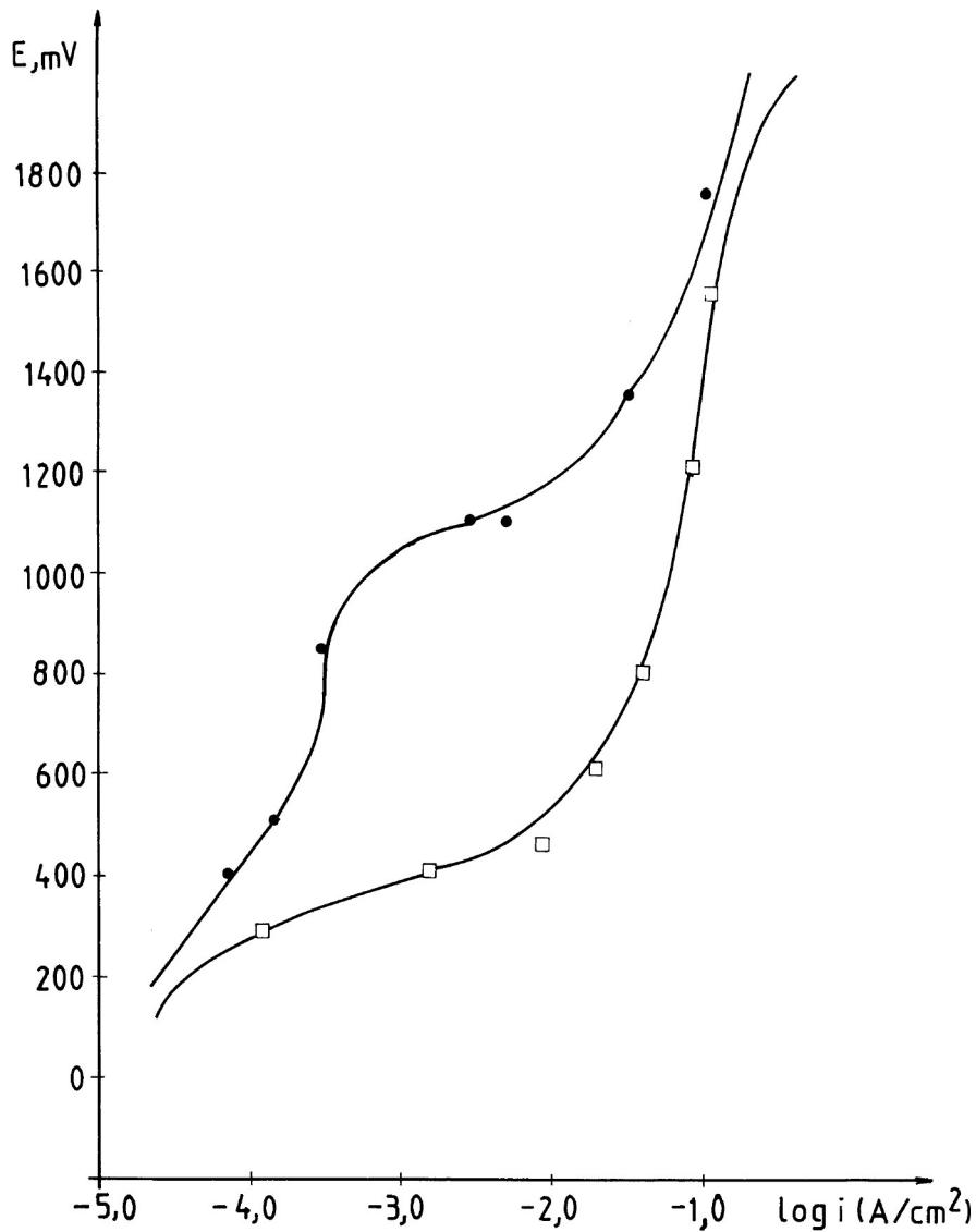
Figure 3. Anode polarization curves in the 50 wt.% \text{Ca(OCl)}_2 suspension where: (●) - steel Č 4574, (□) steel Č 4583.
