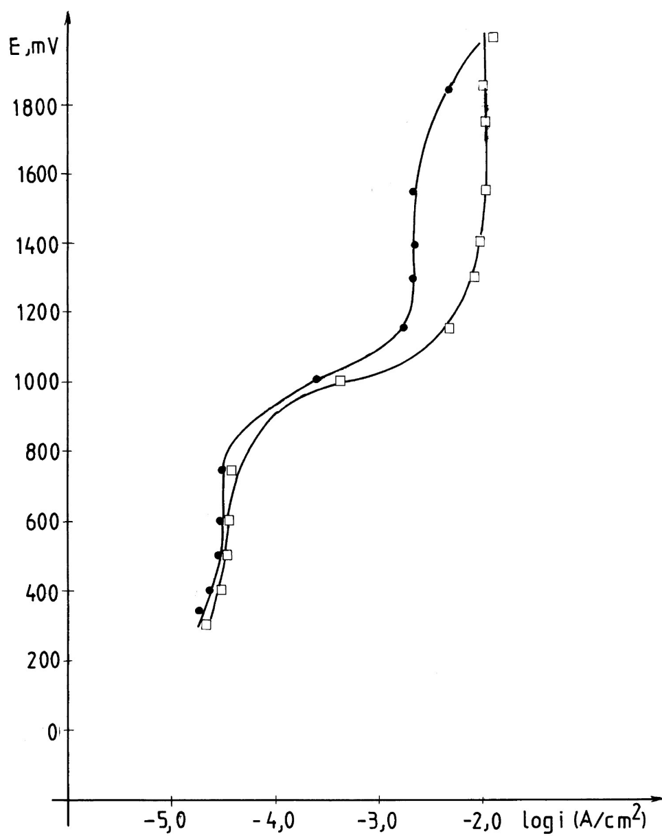
Figure 5. Anode polarization curves in the 1 wt.% \text{Ca(OCl)}_2 suspension where: (●) - steel Č 4574, (□) steel Č 4583.
