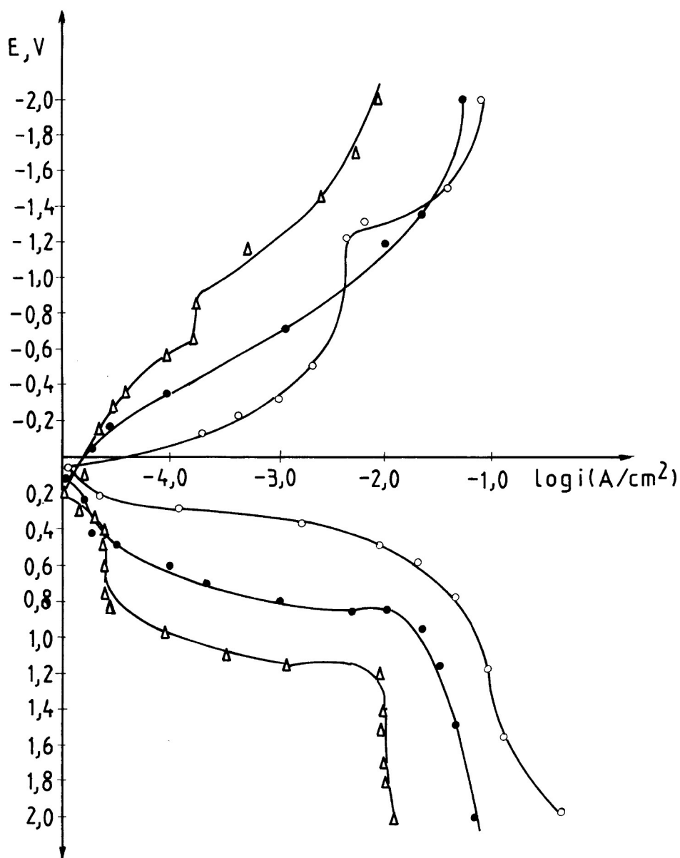
Figure 1. Potentiodynamic curves for steel Č 4574 in tested corrosive media where: (o) E_r = 60\text{mV} , (•) E_r = 120\text{mV} , ( \Delta ) E_r = 186\text{mV} , i.e. (o) - 50 wt. % suspension, (•) 10 wt. % solution i ( \Delta ) 1 wt. % solution.
