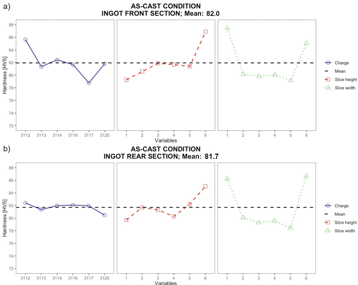
Figure 2. Effect of individual variables on mean HV5 hardness in the as-cast condition: (a) ingot front section; (b) ingot rear section
