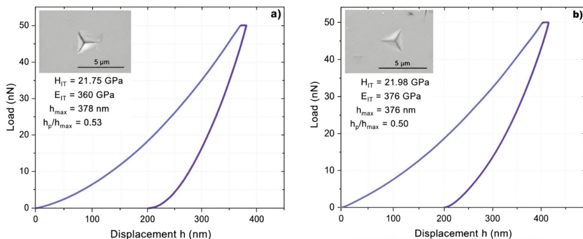
Figure 10. SEM images of indents and nanoindentation curves for two processing parameters (a) steel borided at 1223 K for 6 h and (b) steel borided at 1273 K for 4 h
