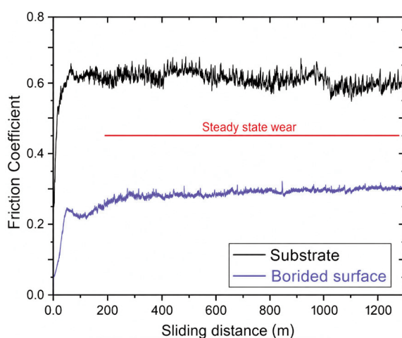
Figure 11. Evolution of the friction coefficient as a function of sliding distance for two ASTM A29 steel surfaces: borided (1273 K for 8 h) and unborided
