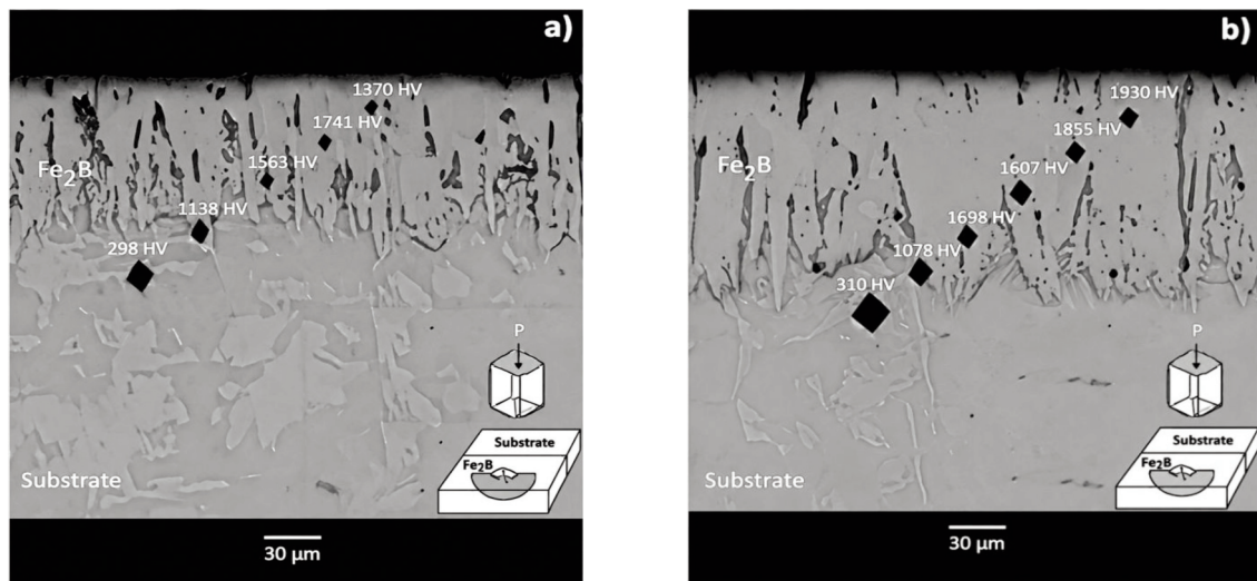
Figure 8. Optical images showing the Vickers indents along the boride layers for two different loads and processing parameters : (a) 6 h at 1223 K under a load of 50 gf, and (b) 4 h at 1273 K under a load of 100 gf
