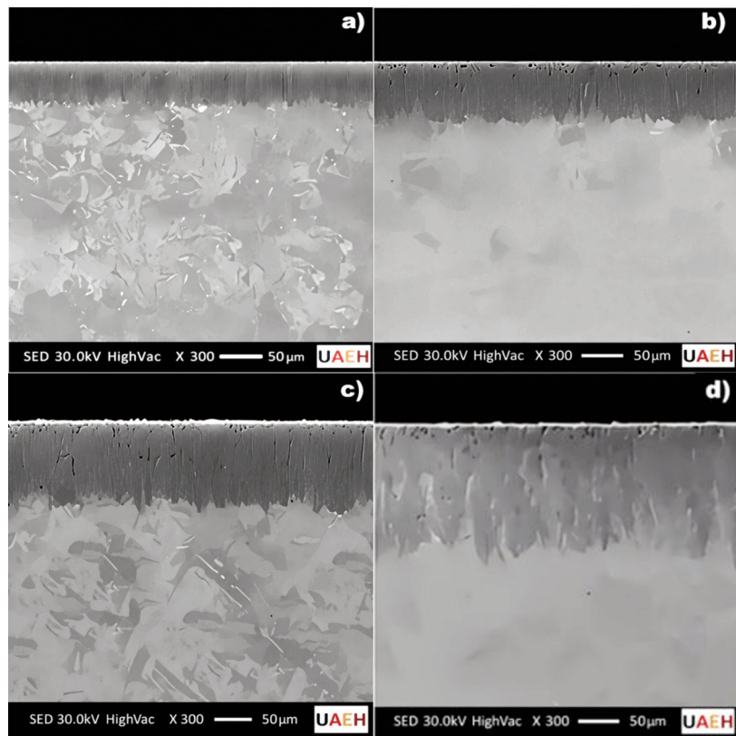
Figure 5. SEM micrographs showing the Fe,B layers on the ASTM A29 steel obtained at different temperatures for 6 h: (a) 1123 K, (b) 1173 K, (c) 1223 K, and (d) 1273 K
