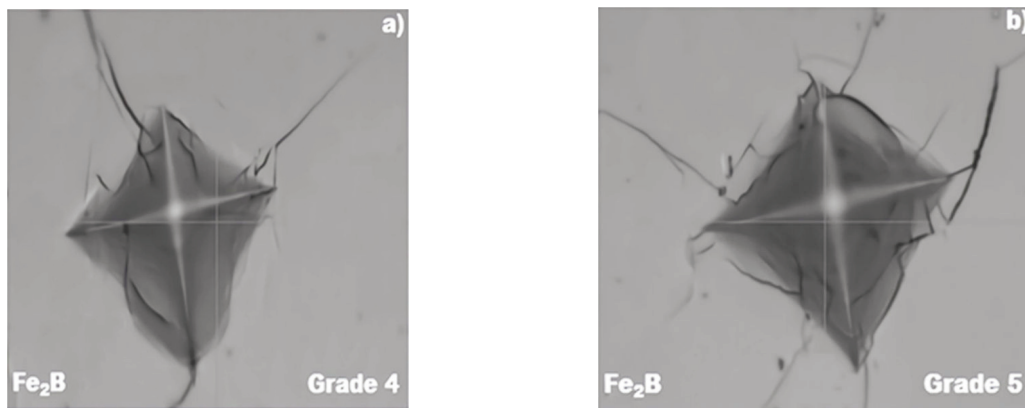
Figure 9. Behaviour of \text{Fe}_2\text{B} layers formed on ASTM A29 steel (1273 K for 4 h) under two applied loads using a Vickers indenter: (a) 50 gf and (b) 100 gf
