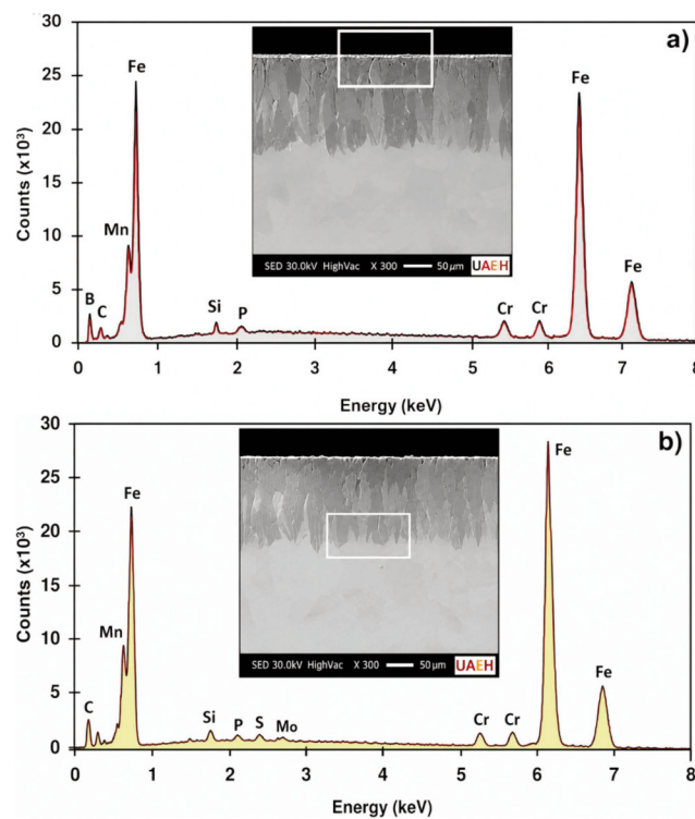
Figure 6. SEM images of cross-sections of boride layers obtained at 1273 K for 8 h along with the EDS analyses in two distinct locations: (a) near the top surface, (b) at the (boride layer/substrate) interface
