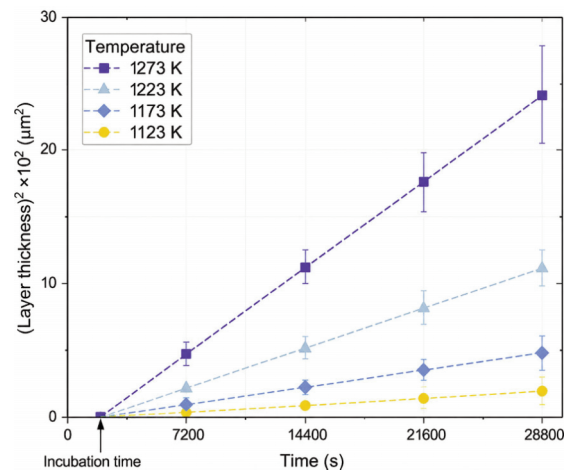
Figure 13. Kinetic analysis of \text{Fe}_2\text{B} layer growth over time
