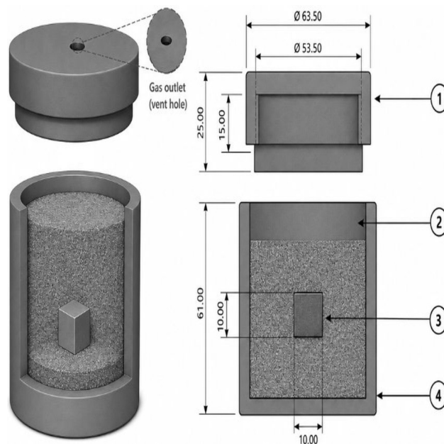
Figure 1. Experimental setup used for the pack-boriding treatment. It includes: (1) a lid with a small opening for the release of gaseous species, (2) the powder mixture used, (3) the sample to be treated, and (4) the main cylindrical body of the container. All dimensions are given in mm
