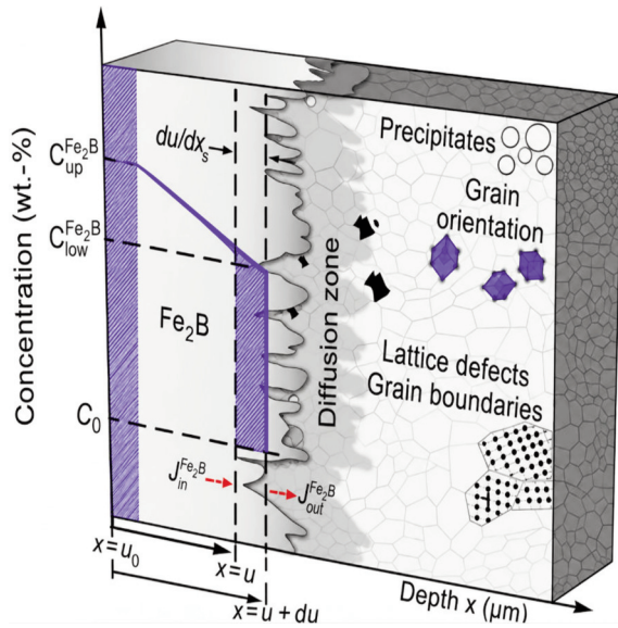
Figure 4. The generated \text{Fe}_2\text{B} layer along with the B distribution across it
