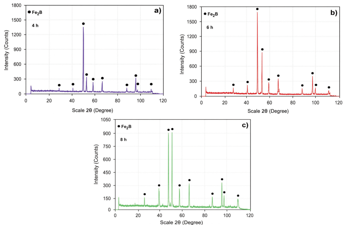
Figure 7. XRD diffractograms of borided surfaces of ASTM A29 steel at 1273 K for different treatment times: (a) 4 h, (b) 6 h, and (c) 8 h
