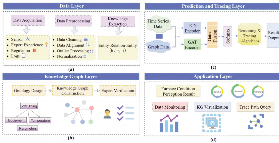
Figure 10. System architecture diagram
