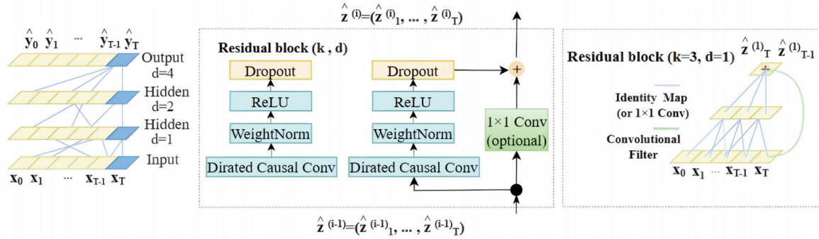
Figure 5. Schematic diagram of the TCN residual block structure
