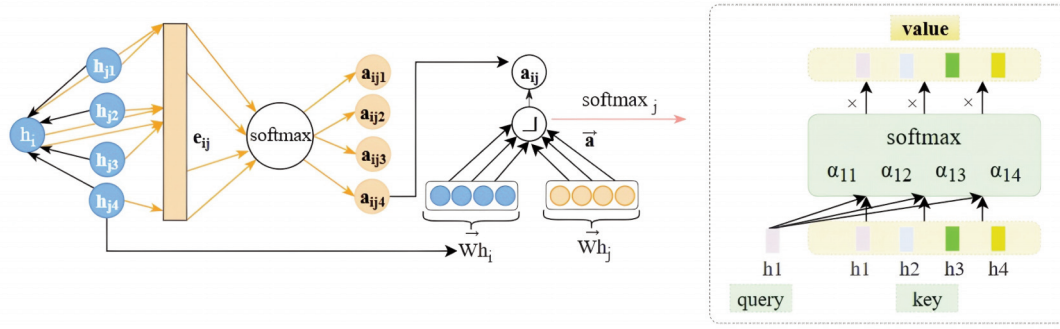
Figure 6. Schematic diagram of the graph attention mechanism computation
