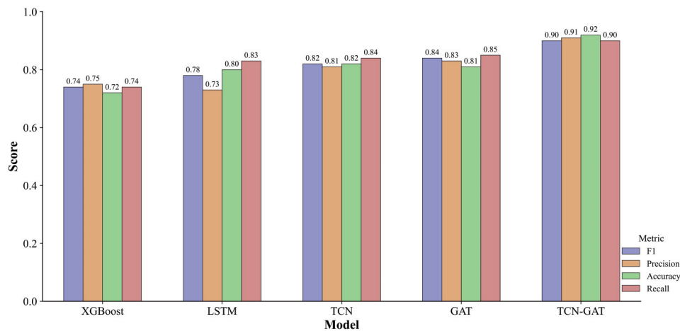
Figure 7. Performance comparison of different models
