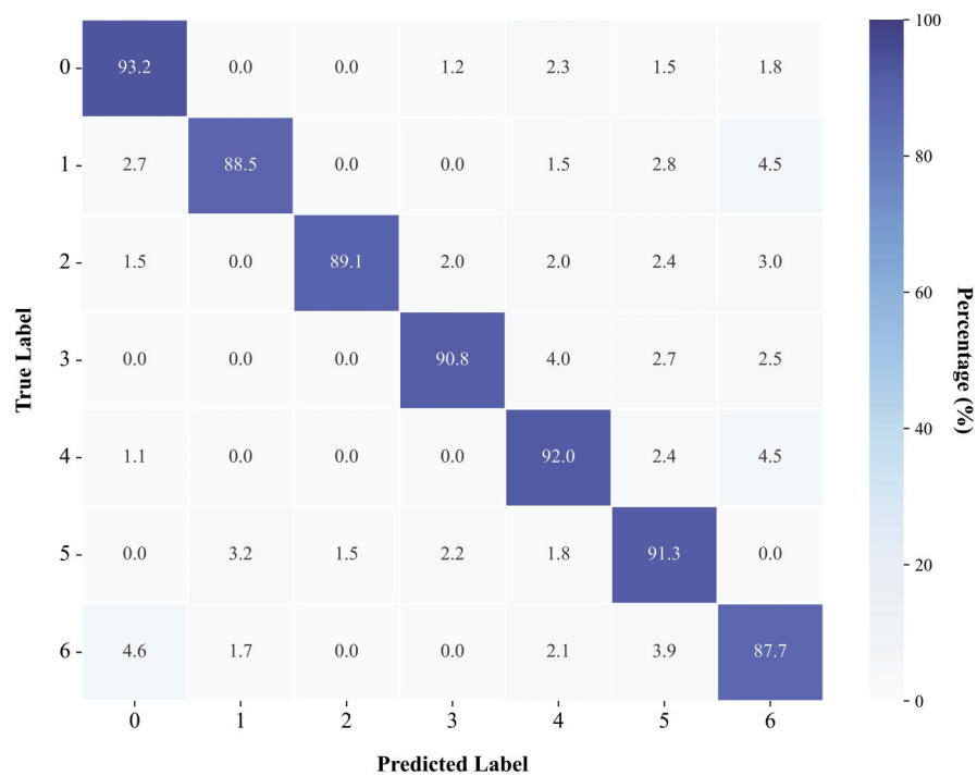
Figure 8. Visual analysis of confusion matrix
