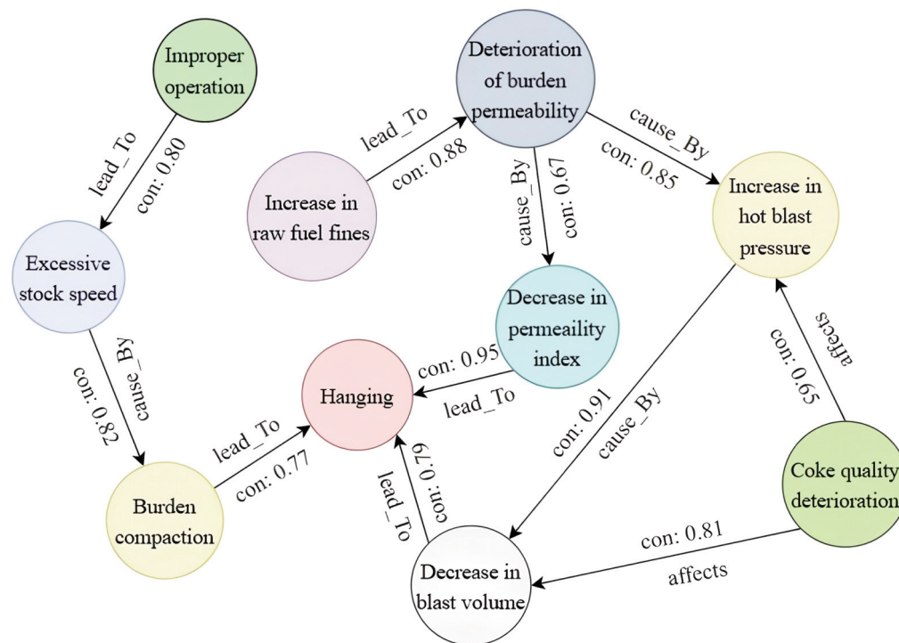
Figure 9. Example of a root cause chain for hanging
