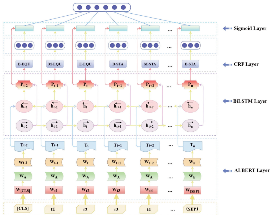
Figure 2. Architecture of the ALBERT-BiLSTM-CRF knowledge extraction model
