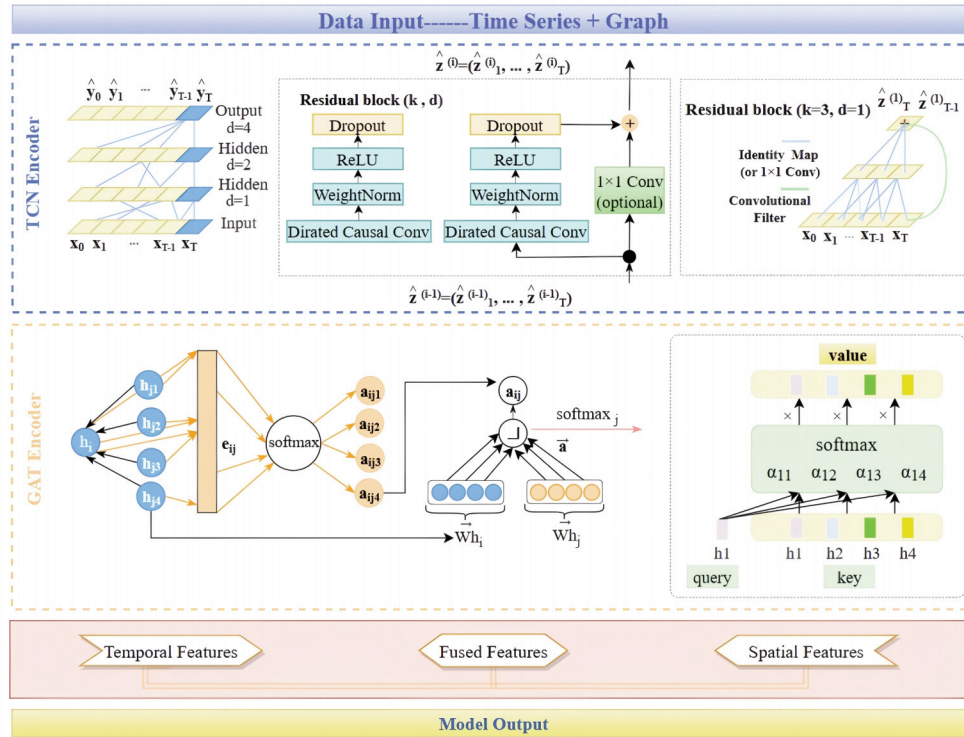
Figure 4. Overall architecture of the proposed model
