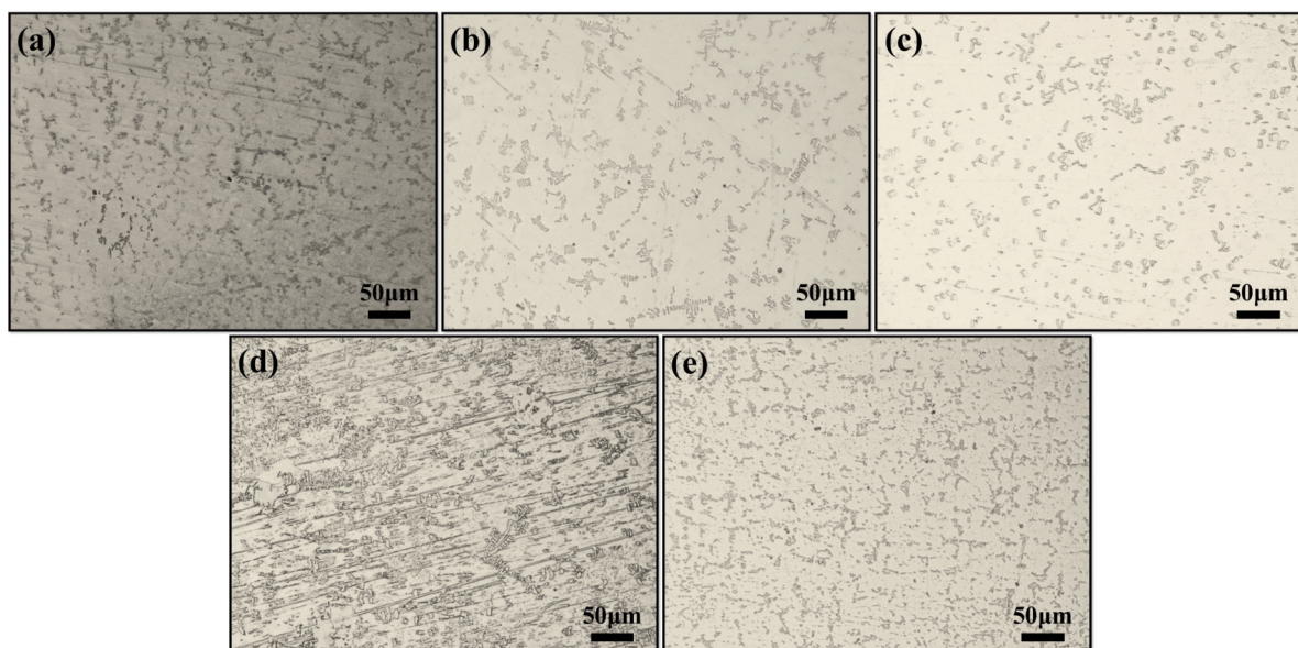
Figure 2. The metallographic structure of the Ni49.5Ti38.5Zr12 alloy samples in the as-homogenized state and after annealing at different temperatures: (a) as-homogenized, (b) 500 °C, (c) 600 °C, (d) 700 °C, and (e) 800 °C
