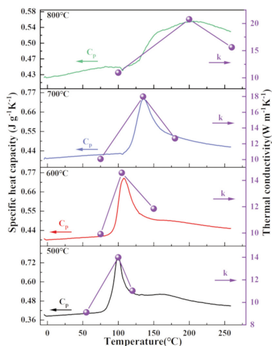
Figure 5. The specific heat capacity and thermal conductivity of the Ni49.5Ti38.5Zr12 alloy after annealing at different temperatures
