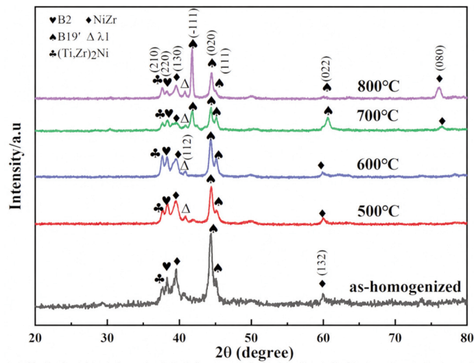
Figure 1. The XRD patterns of the Ni49.5Ti38.5Zr12 alloy in the as-homogenized state and after annealing at different temperatures
