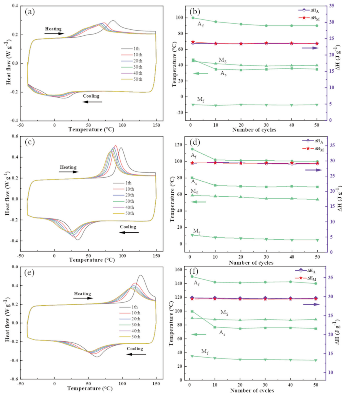
Figure 6. The thermal cycling curves and corresponding phase transformation curves of the Ni 49.5 Ti 38.5 Zr 12 alloy at different annealing temperatures: (a) Thermal cycling curve at 500 °C (b) Phase transformation temperature curve at 500 °C (c) Thermal cycling curve at 600 °C (d) Phase transformation temperature curve at 600 °C (e) Thermal cycling curve at 700 °C (f) Phase transformation temperature curve at 700 °C
