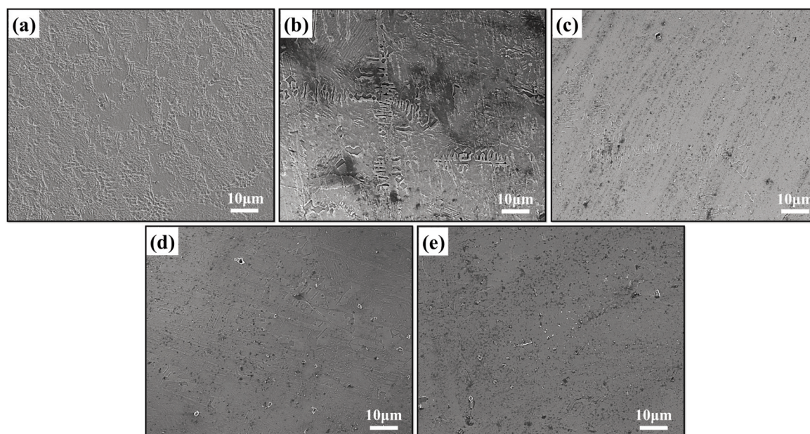
Figure 3. The SEM images of the Ni49.5Ti38.5Zr12 alloy samples in the as-homogenized state and after annealing at different temperatures: (a) as-homogenized, (b) 500 °C, (c) 600 °C, (d) 700 °C, and (e) 800 °C
