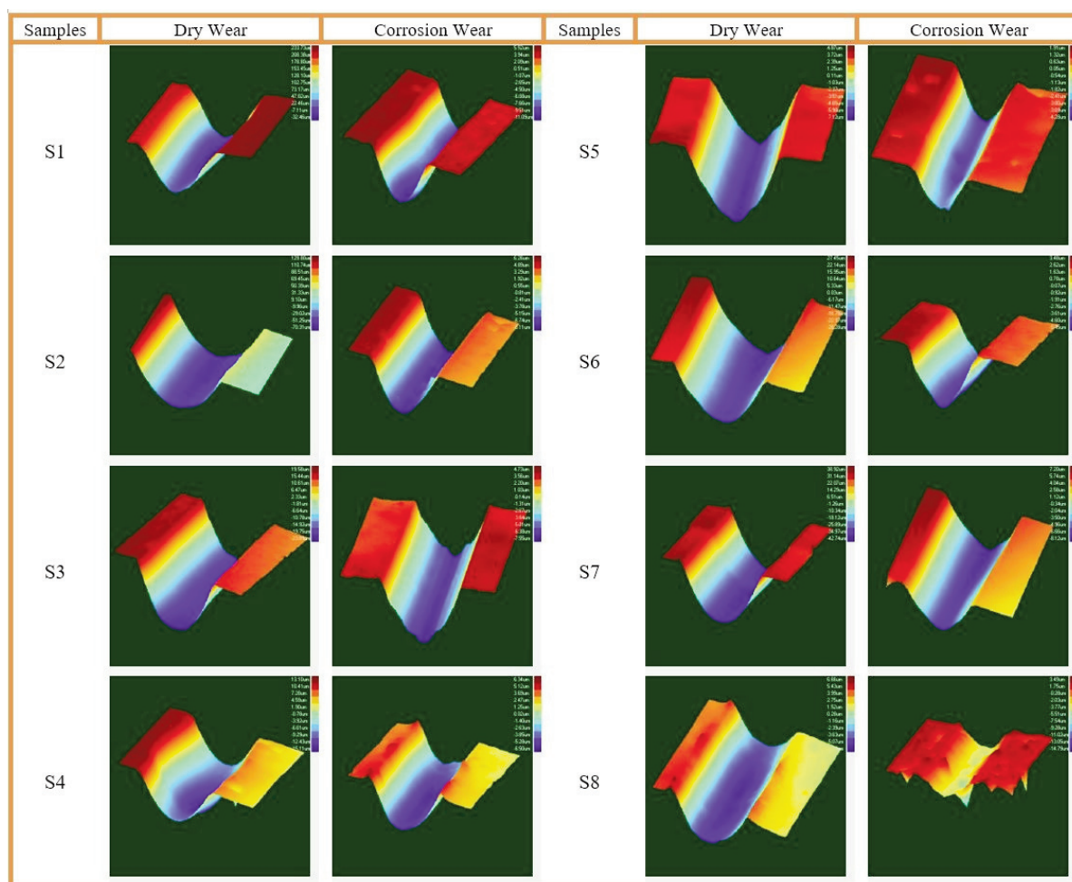
Figure 8. Surface topographies of samples worn in dry and corrosive environments at 30 N load
