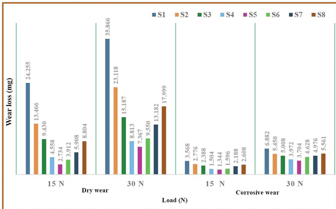
Figure 3. Weight wear amounts in dry sliding and corrosive sliding
