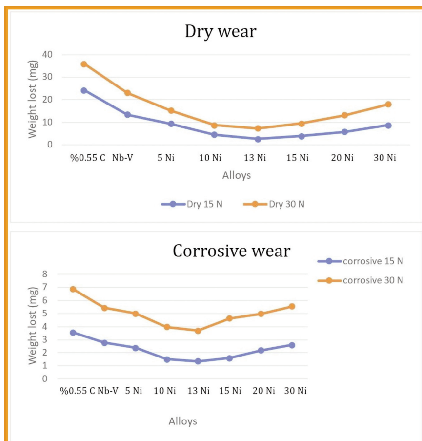
Figure 4. Weight loss graphs
