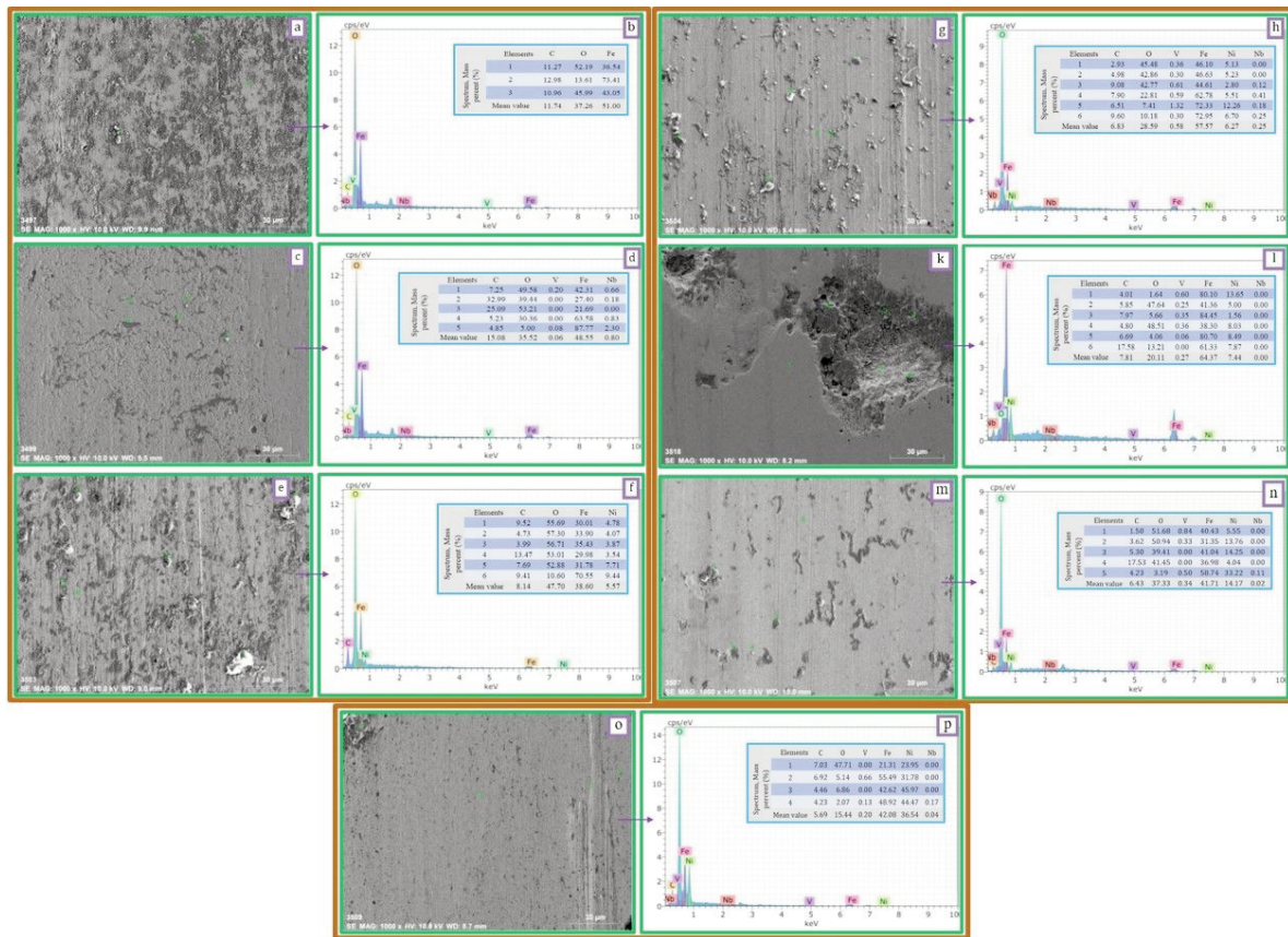
Figure 6. EDX analyses taken from dry wear surfaces at 30 N load; a) S1 surface points, b) S1 EDX peaks and elemental composition by weight, c) S2 surface points, d) S2 EDX peaks and elemental composition by weight, e) S3 surface points, f) S3 EDX peaks and elemental composition by weight, g) S4 surface points, h) S4 EDX peaks and elemental composition by weight, i) S6 surface points, j) S6 EDX peaks and elemental composition by weight, k) S7 surface points, l) S7 EDX peaks and elemental composition by weight, m) S8 surface points, n) S8 EDX peaks and elemental composition by weight
