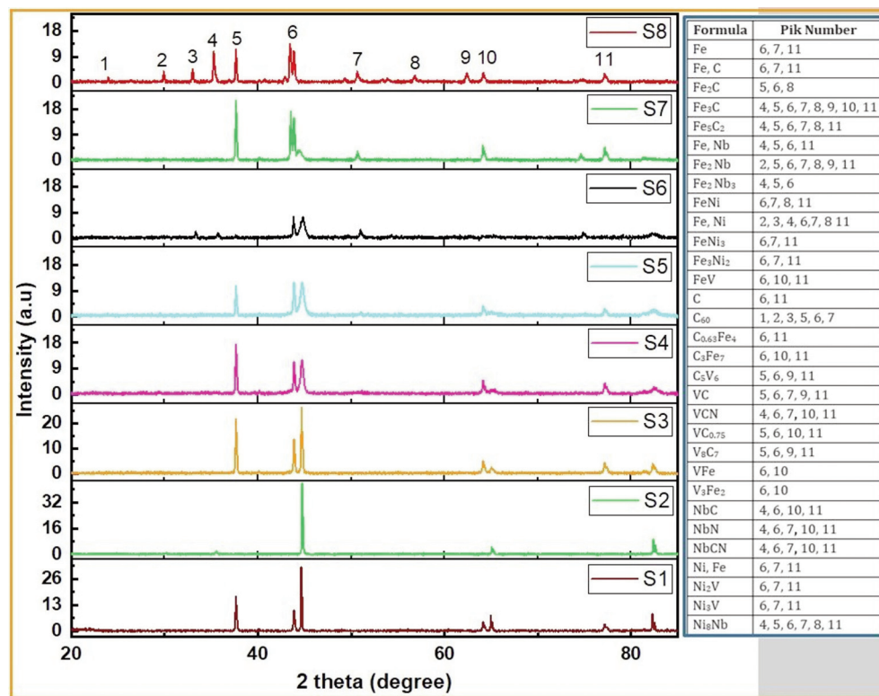
Figure 7. XRD pattern of the samples
