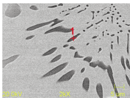
Figure 8. Scanning image of alloy P2 (17.7 wt.% V+4.5 wt.% W); lamellar and eutectic carbides in the alloy matrix
