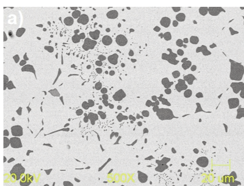
Figure 13. Scanning image of alloy P3 (17.9 wt.% V+0.1 wt.% W); a) oval and spherical carbides evenly distributed in the alloy matrix, b) marked locations of analysis
