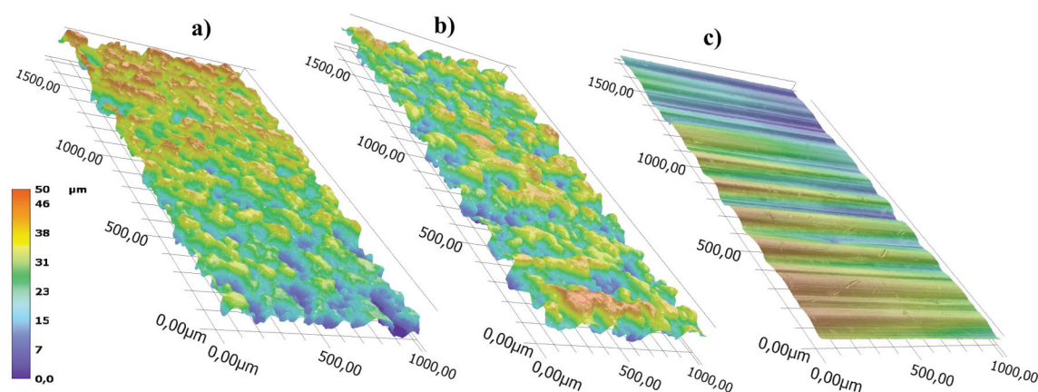
Figure 17. Comparison of wear surface profiles obtained in the Miller test: a) martensitic alloy P2 with the addition of 17.7 wt.% V + 4.5 wt.% W, b) martensitic alloy P3 with the addition of 17.9 wt.% V + 0.1 wt.% W, c) reference specimen cast GX70CrMnSiNiMo2 steel
