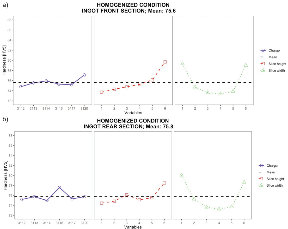
Figure 3. Effect of individual variables on mean HV5 hardness in the homogenized condition: (a) ingot front section; (b) ingot rear section
