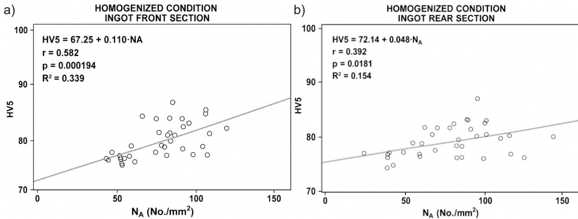
Figure 5. Correlation between number of grains per unit area ( N_A ) and mean HV5 hardness in the homogenized condition: (a) ingot front section; (b) ingot rear section
