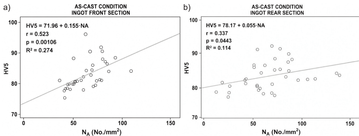
Figure 4. Correlation between number of grains per unit area ( N_A ) and mean HV5 hardness in the as-cast condition: (a) ingot front section; (b) ingot rear section
