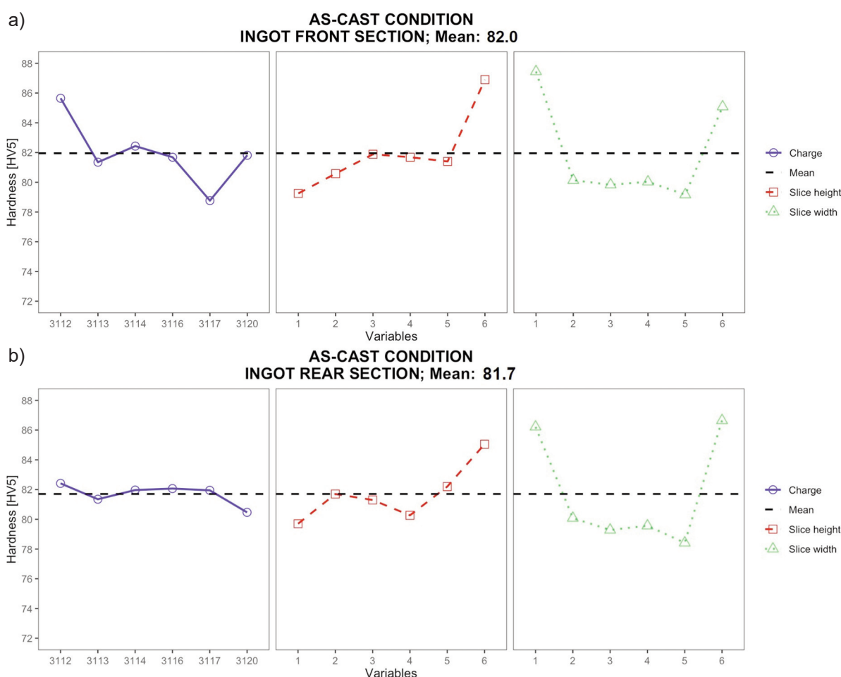
Figure 2. Effect of individual variables on mean HV5 hardness in the as-cast condition: (a) ingot front section; (b) ingot rear section
